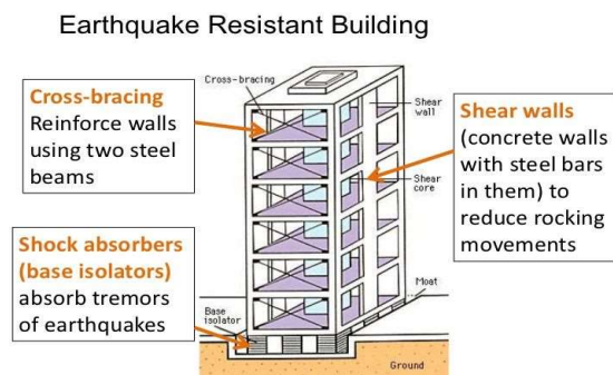
Figure 2e Shows components of a typical earthquake resistant building
